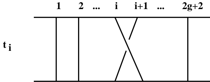
Figure 4.1: Loops generating B_{2g+2} .
